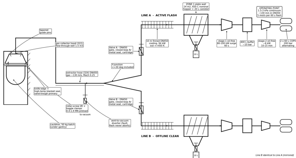
FIG. 7 — THE CATCH (TRAIN LAYOUT). The cold-trap train behind the hood: the DN450 burst line at 1.5 to 3 kPa, the 650 °C plate wall in eight chevron banks, the finned cooling section, the argon gate valves at the Y-junction, and the compression skids to buffer and bottle.
