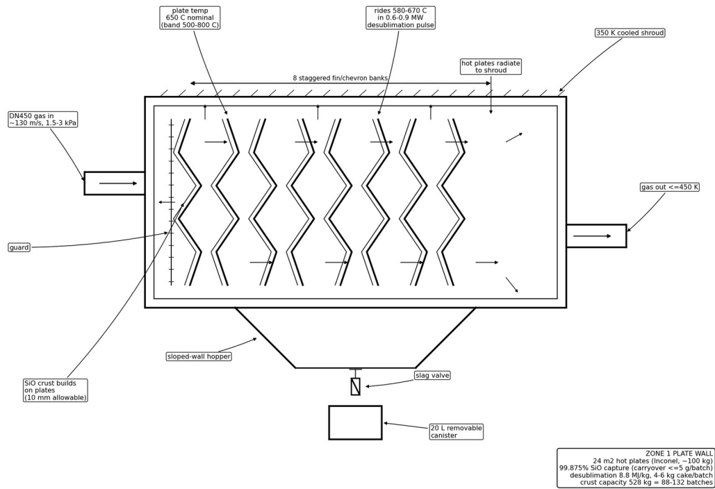
FIG. 8 — THE PLATE WALL (SECTION). SiO desublimes as a solid crust on the hot plates — 24 m 2 of Inconel at 650 °C, 8.8 MJ per kilogram, 99.875 percent capture, 528 kg of crust between cleanouts.
